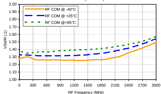
VSWR @ Vdd=+3V over Temperature RF COM (State 3*)
