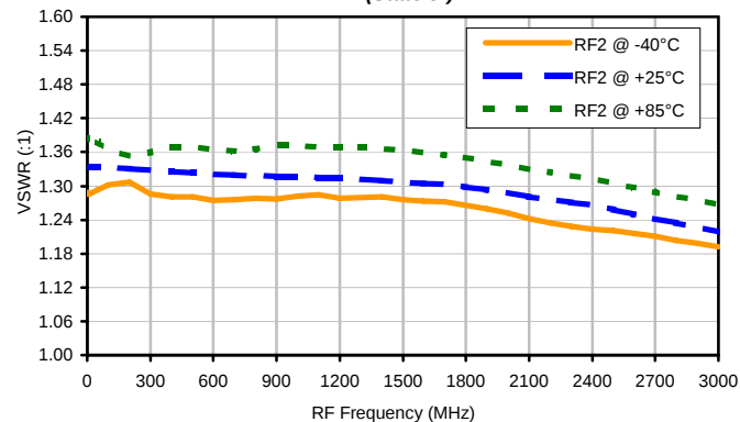
VSWR @ Vdd=+3V over Temperature RF2 (State 3*)
