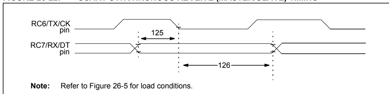
FIGURE 26-22: USART SYNCHRONOUS RECEIVE (MASTER/SLAVE) TIMING
