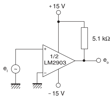
Figure 17. Split-supply applications - zero crossing detector
