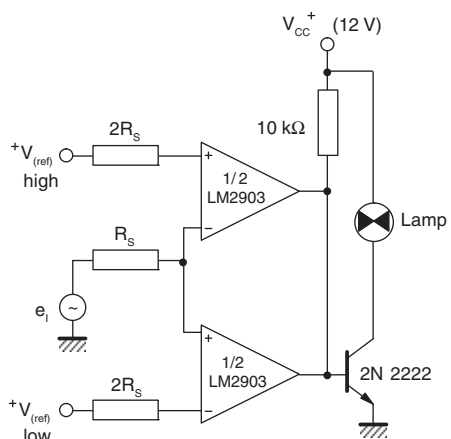
Figure 16. Limit comparator
