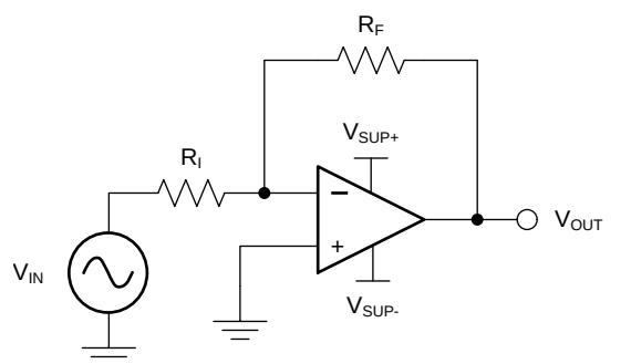
Figure 38. Application Schematic
