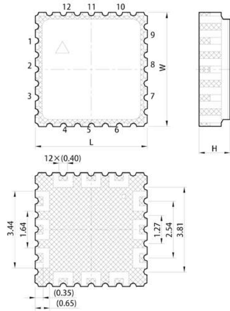
QFN 5X5
