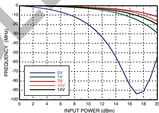
F_{center} vs. Input Power V_{fctl} = V_{nctl}
