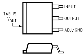
Pin Functions
