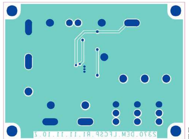
Figure 92. PCB Layout, Bottom
