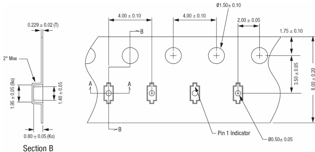
Figure 4. SC-79 Package Dimension Drawing
