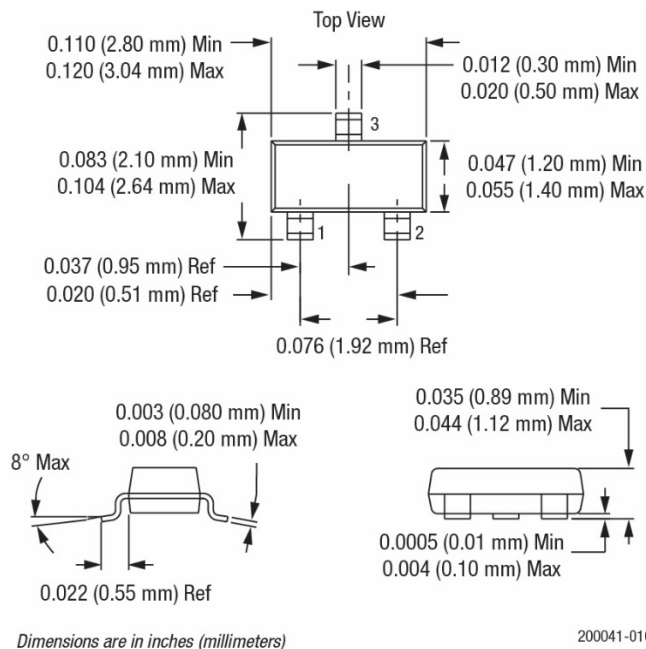
Figure 8. SOT-23 Package Dimension Drawing
