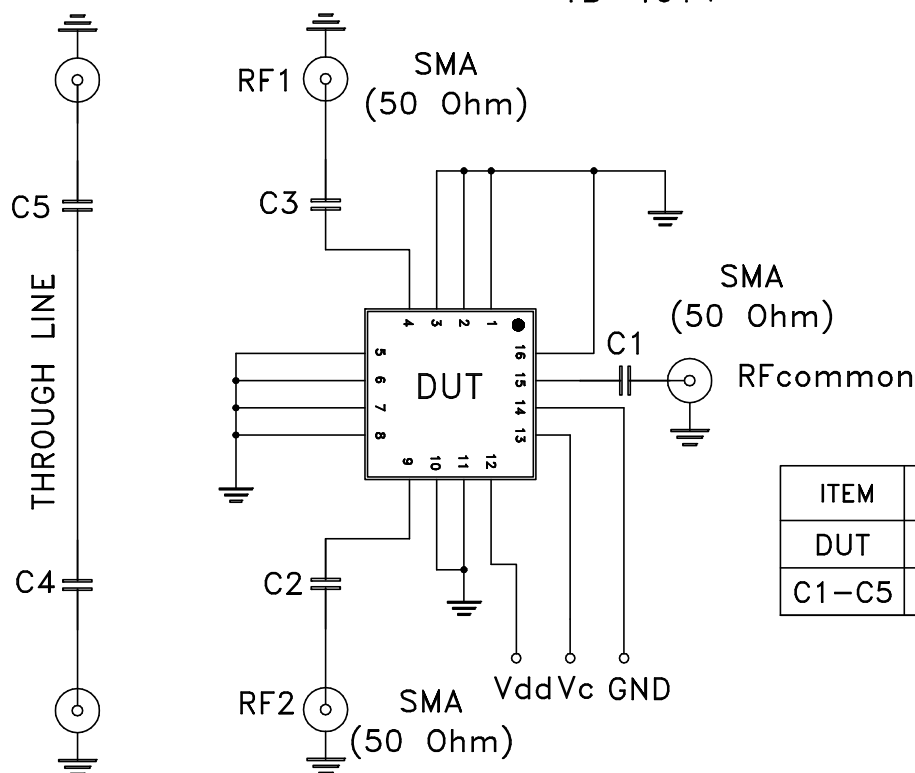
Schematic Diagram
