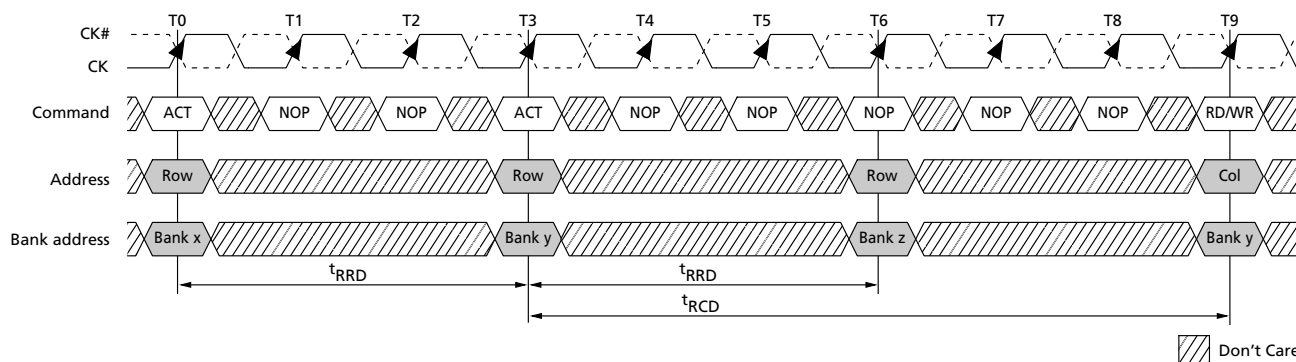
Figure 44: Example: Meeting t_{\text{RRD}}(\text{MIN}) and t_{\text{RCD}}(\text{MIN})
