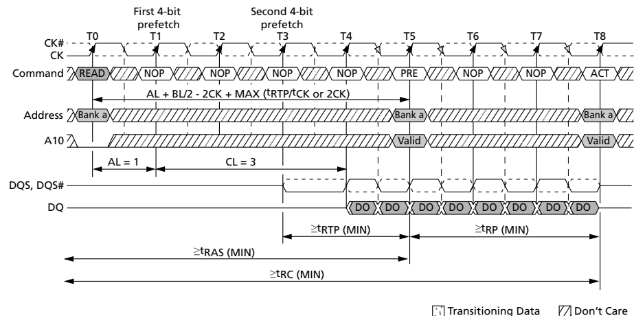
Figure 52: READ-to-PRECHARGE – BL = 8
