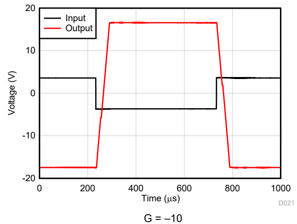
Figure 6-28. Overload Recovery
