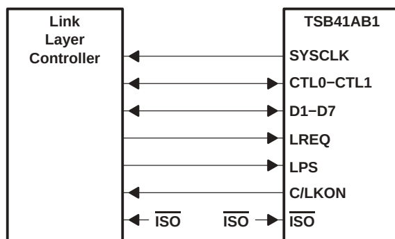
Figure 18. PHY-LLC Interface
