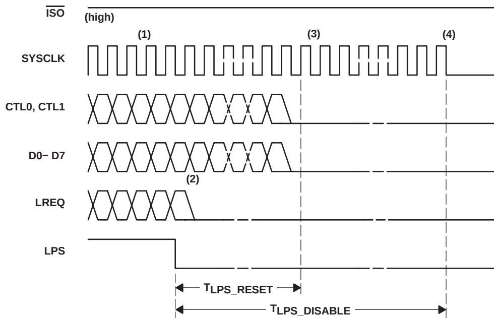
Figure 30. Interface Disable, \overline{\text{ISO}} High
