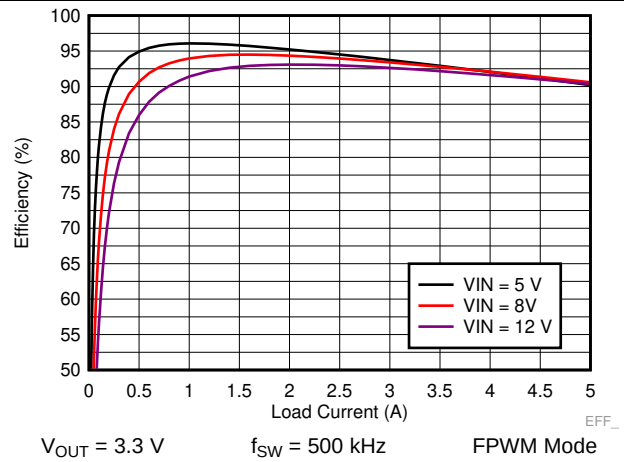
Figure 28. LM73605 Efficiency
