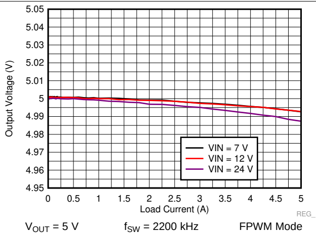
Figure 44. LM73605 Load and Line Regulation
