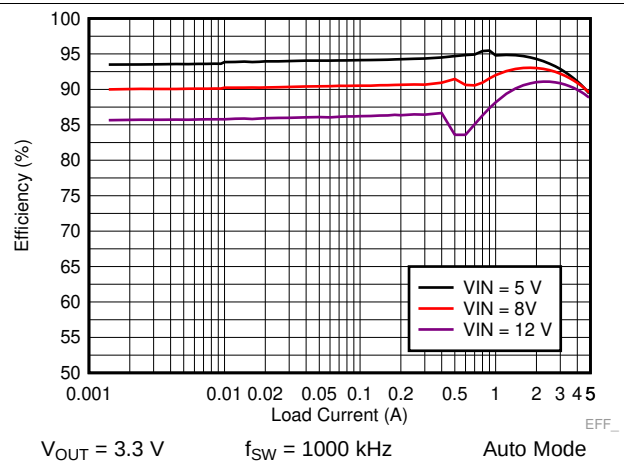
Figure 32. LM73605 Efficiency
