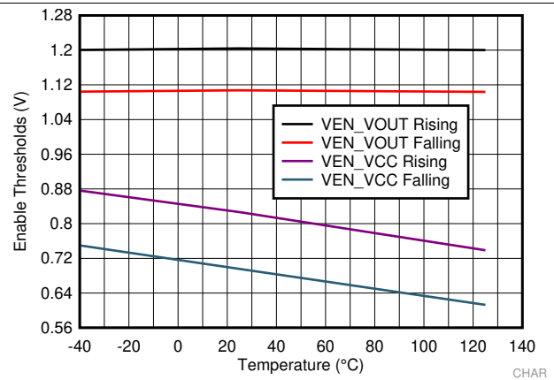
Figure 8. Enable Thresholds
