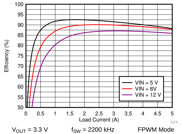
Figure 30. LM73605 Efficiency
