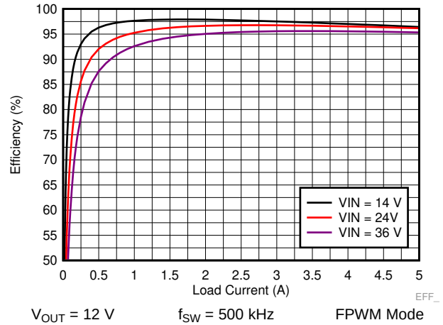
Figure 40. LM73605 Efficiency
