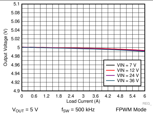
Figure 42. LM73606 Load and Line Regulation
