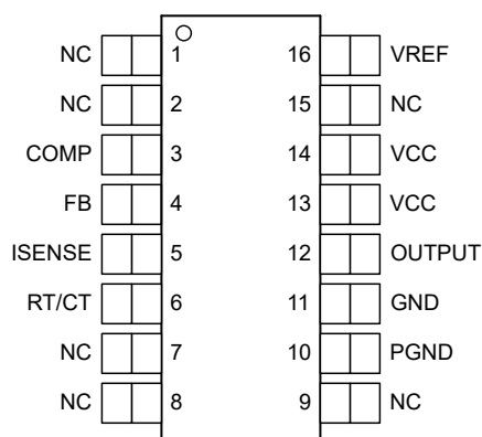
Figure 5-4. SOIC Package, 16-Pin DW (Top View)
