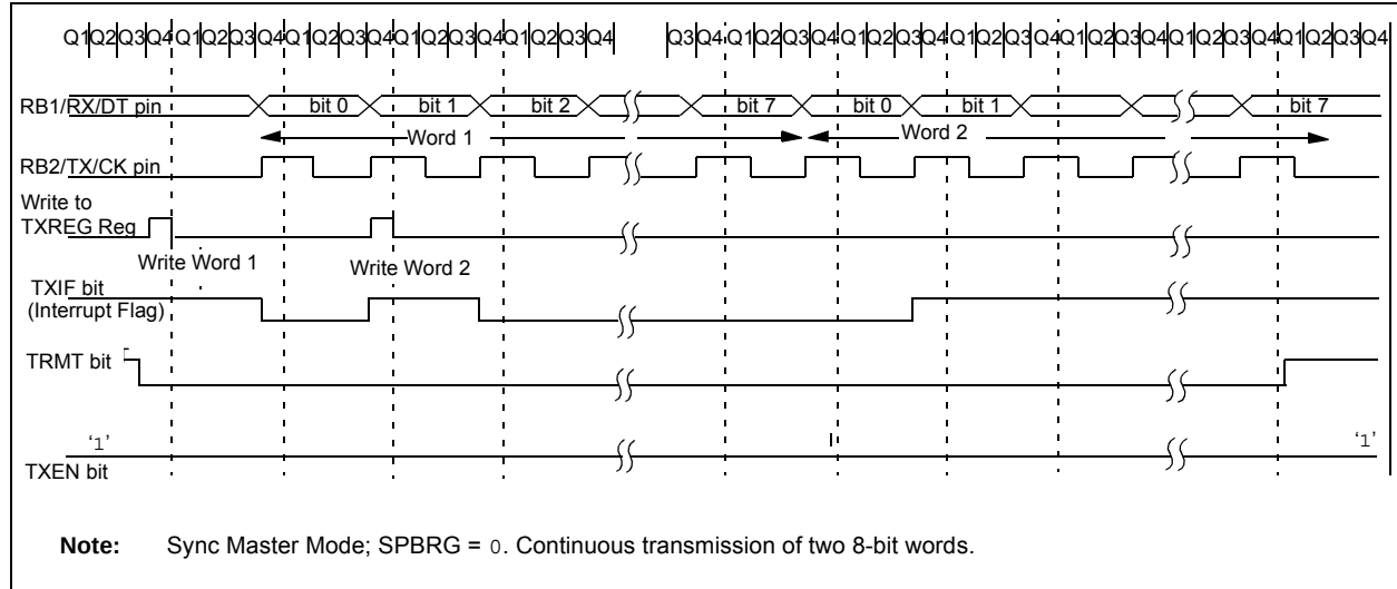
FIGURE 12-8: SYNCHRONOUS TRANSMISSION
