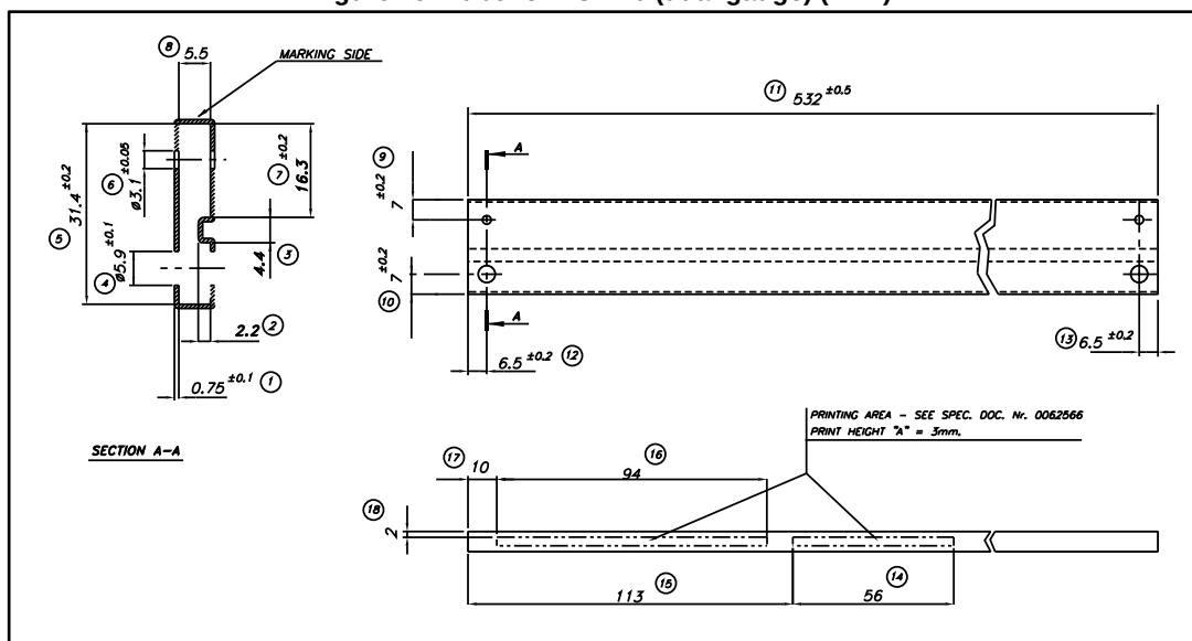
Figure 20: Tube for TO-220 (single gauge) (mm.)
