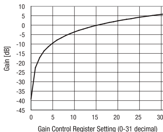
SKY73201 Gain vs. Register Setting
