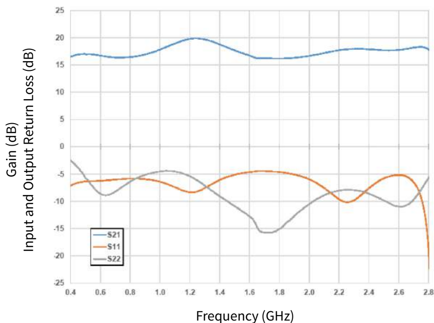
Figure 1. Typical Small Signal Response of CGHV40030F-AMP2 V_{DD} = 50 V, I_{DQ} = 90 mA
