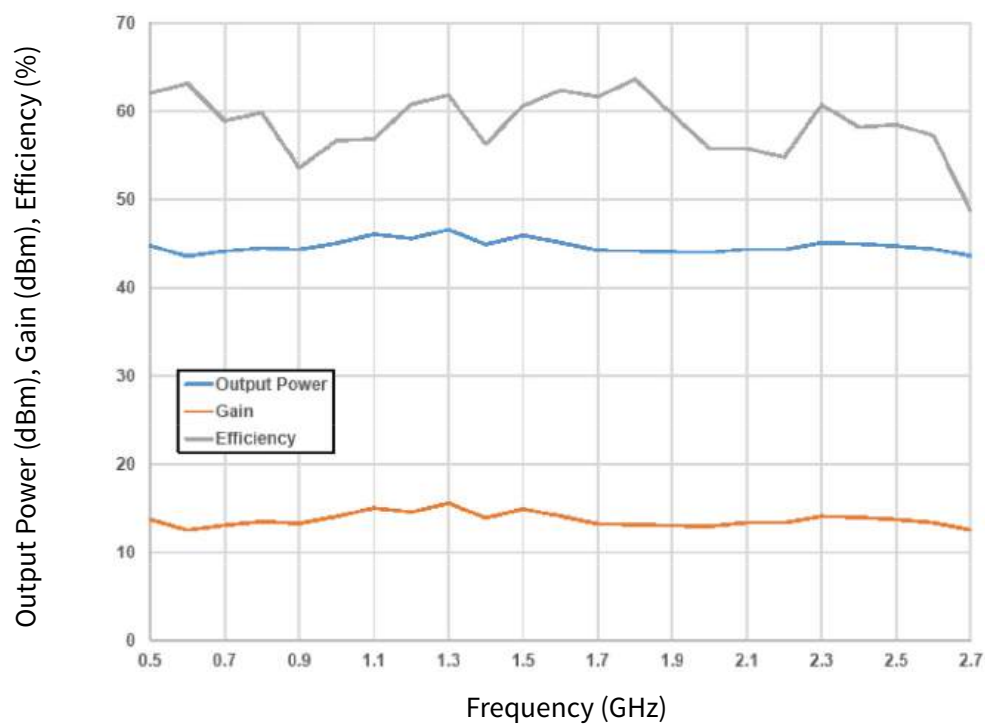
Figure 2. Typical Large Signal Response of CGHV40030F-AMP2 Application Circuit
