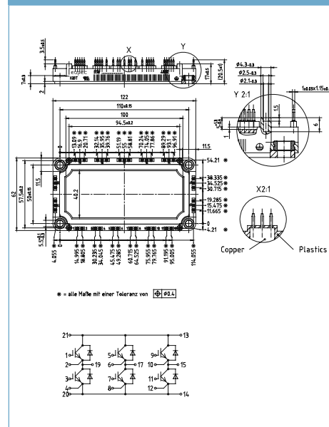
EconoPACK™ 3 A
