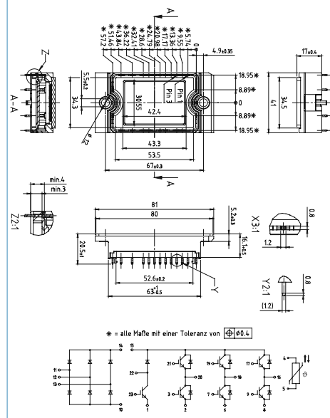
EconoPACK™1 B
