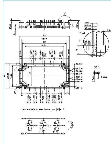
EconoPACK™3 B
