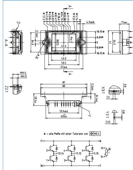
EconoPACK™1 B
