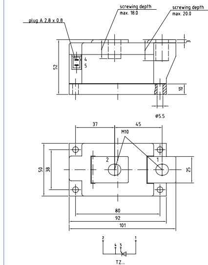
50 mm TP50.1
