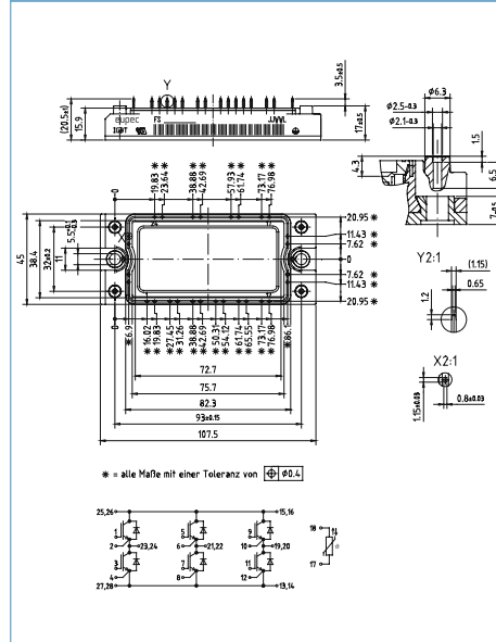
EconoPACK™ 2 B
