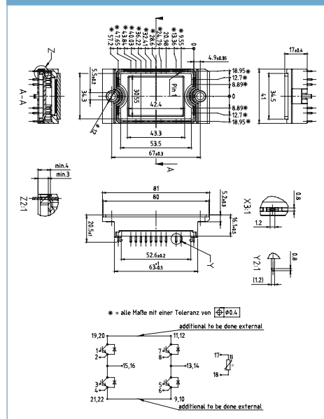
EconoPACK™ 1B FourPACK
