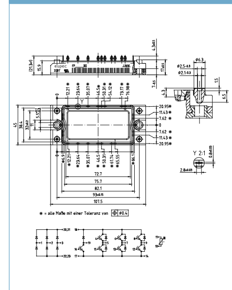
EconoPIM™ 2B PressFIT
