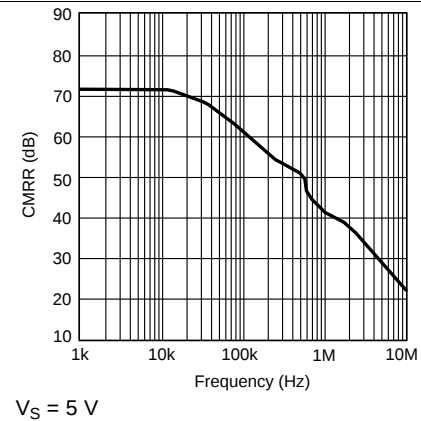
Figure 20. CMRR vs. Frequency
