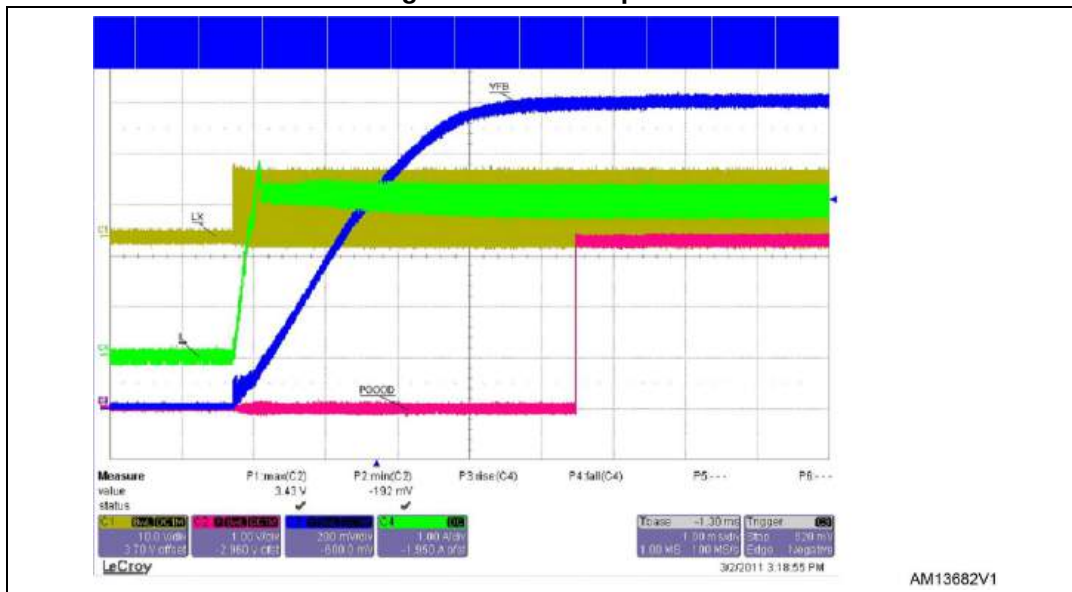
Figure 5. Soft-start phases
