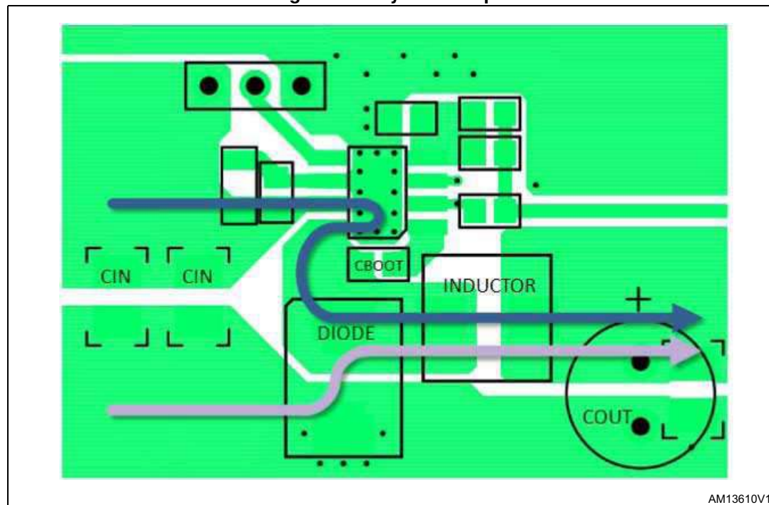
Figure 14. Layout example
