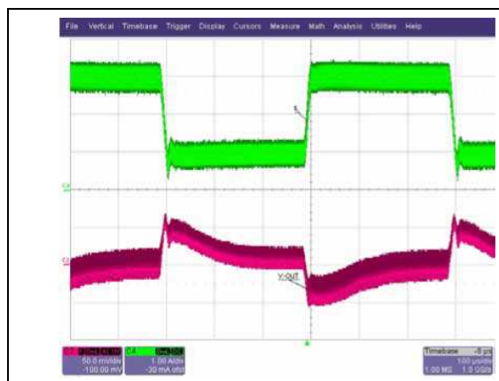
Figure 48. 1 A to 3 A load transient ( V_{IN} 32 V)
