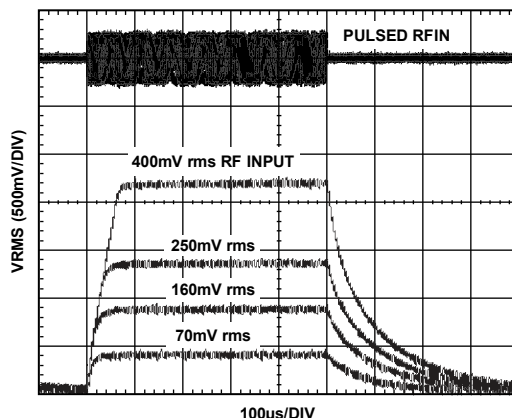
Figure 33. Output Response to Various RF Input Pulse Levels, Supply = 3 V, Frequency = 900 MHz, C_{FLTR} = \text{Open} , C_{OUT} = 0.1 \text{ μF} , R_{OUT} = 1 \text{ kΩ}
