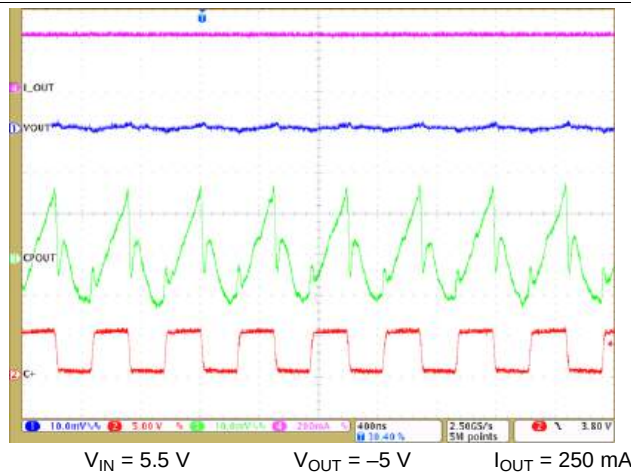
Figure 9. Output Voltage Ripple
