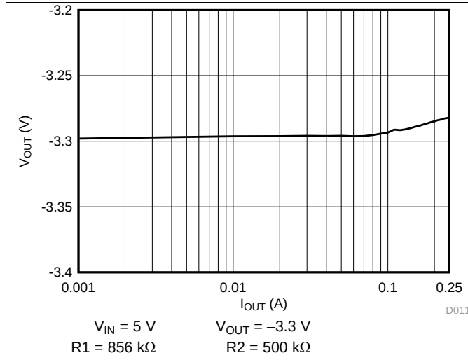
Figure 7. Load Regulation
