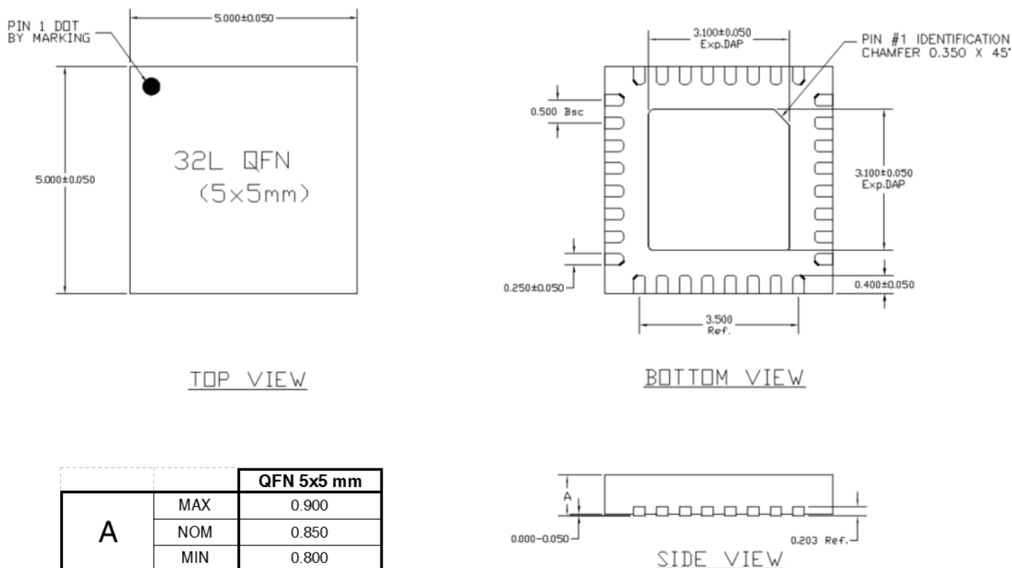
Figure 23 • Package Mechanical Drawing for 5x5 QFN
