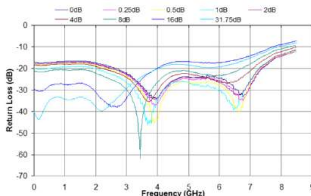
Figure 11 • Input Return Loss vs. Attenuation: T = +25C
