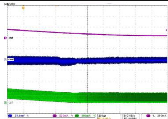
Figure 23. Maximum Output Current
