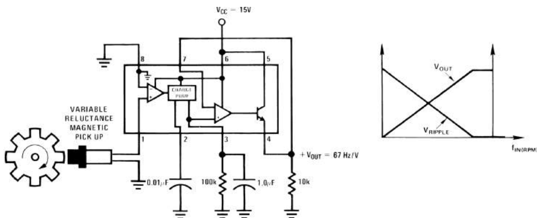
Figure 15. Minimum Component Tachometer Diagram
