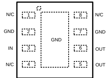
WSO (NGN) Package 8 Pins Top View
