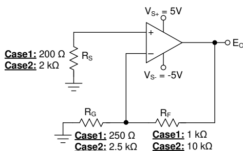
Figure 72. Comparing Noise Contributors for Two Cases With the Amplifier in a Noninverting Gain of 5 V/V
