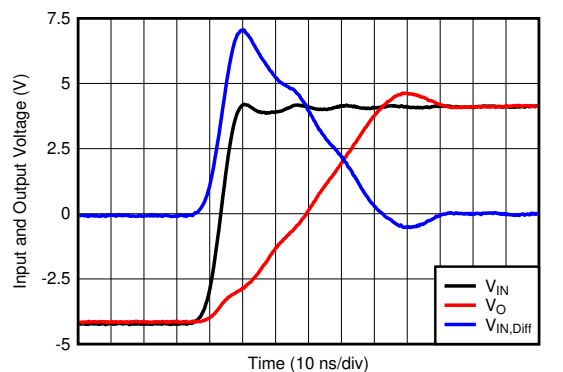
Figure 78. Large-Signal Transient Response Using OPA2810
