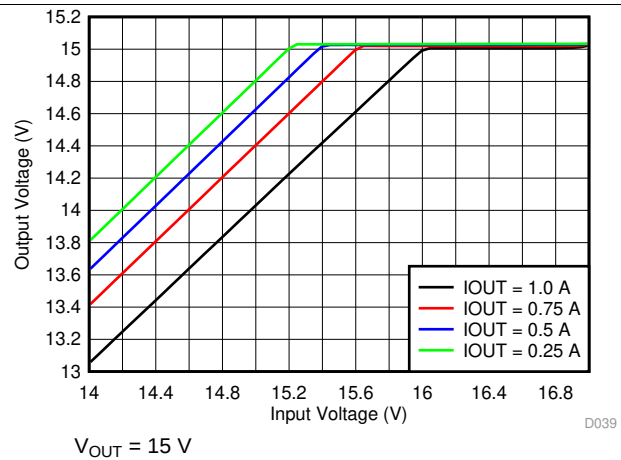
Figure 6. Dropout Voltage
