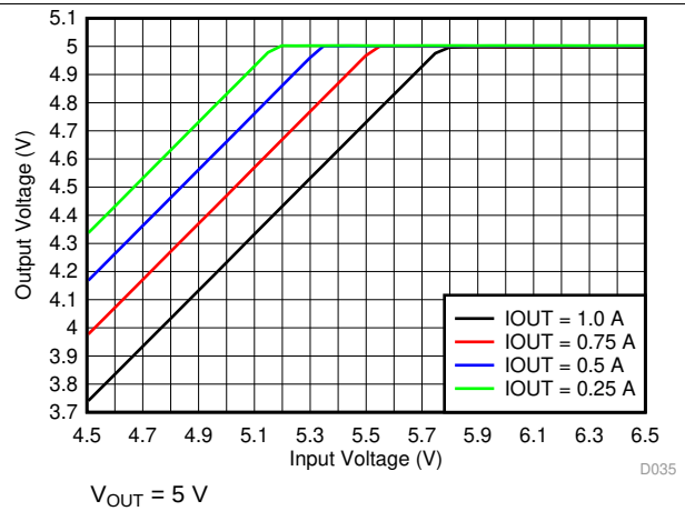
Figure 4. Dropout Voltage
