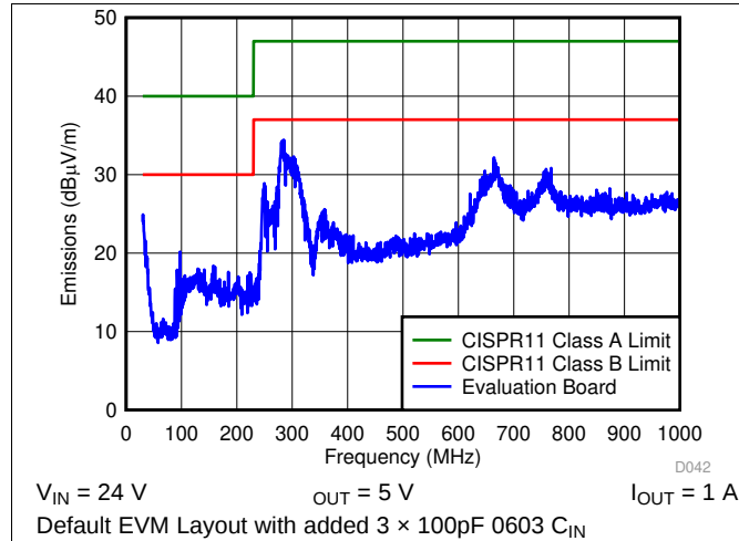
Figure 7. Radiated EMI
