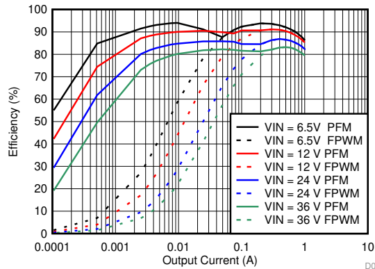
Figure 40. Efficiency
