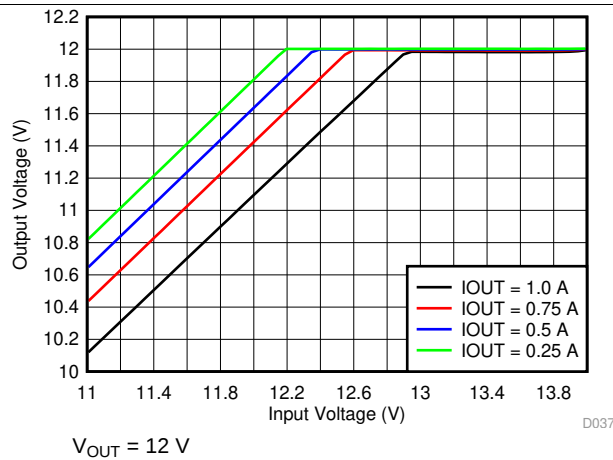
Figure 5. Dropout Voltage
