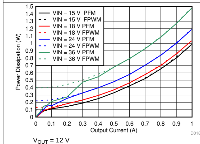
Figure 11. Power Dissipation
