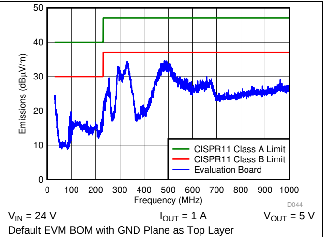
Figure 8. Radiated EMI
