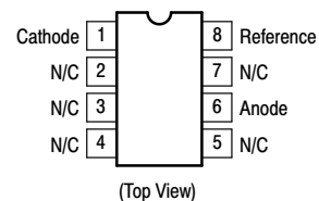
Micro8 ™ DM SUFFIX CASE 846A
