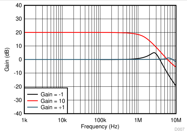
Figure 7-10. Closed-Loop Gain vs Frequency
