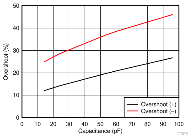
Figure 7-26. Small-Signal Overshoot vs Load Capacitance
