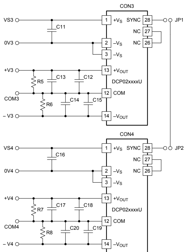
Figure 8-2. PCB Schematic, U Package
