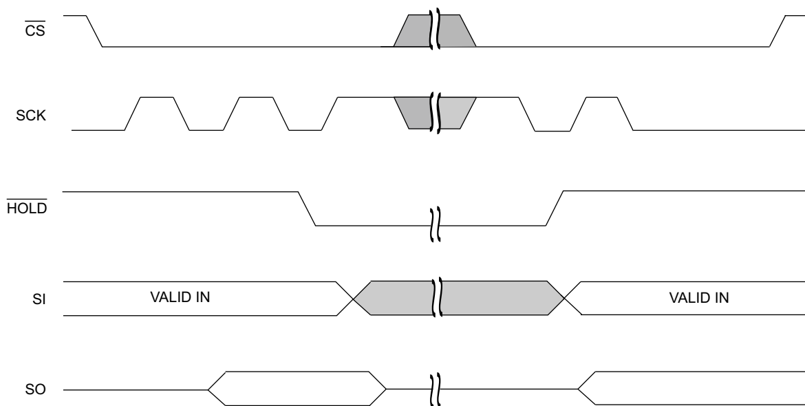
Figure 14. \overline{\text{HOLD}} Operation [2]
