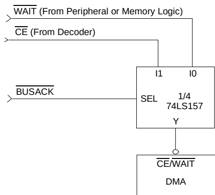
Figure 50. \overline{\text{CE/WAIT}} Multiplexer
