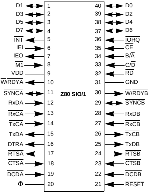
Figure 103. Z80 SIO/1 Pin Functions
