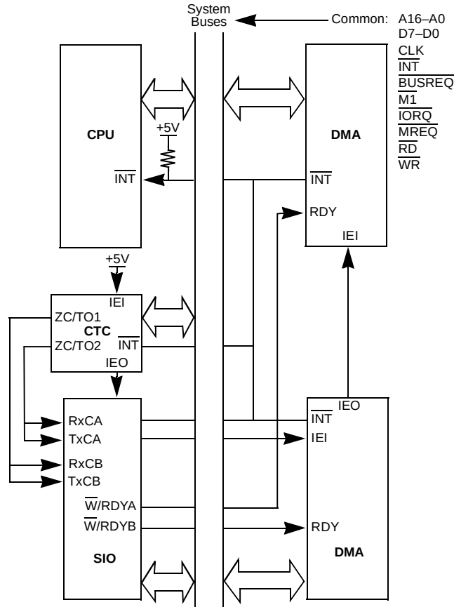
Figure 55. DMA-SIO Environment
