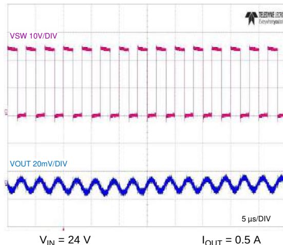
Figure 26. Full-Load Switching
