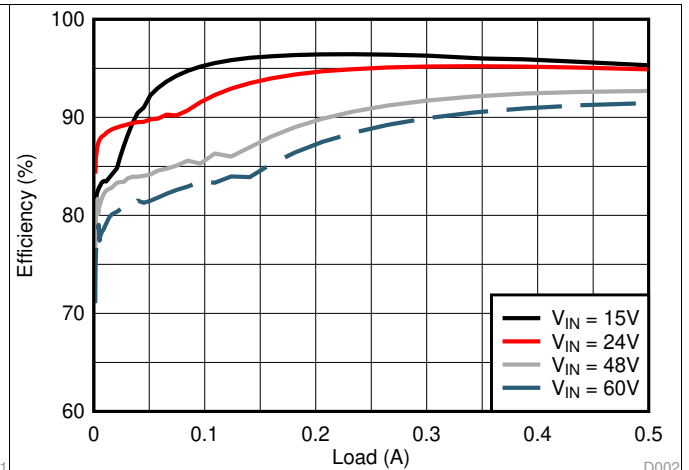
Figure 2. Conversion Efficiency (Linear Scale)
