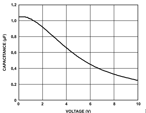
Figure 63. Capacitance vs. Voltage Characteristic
