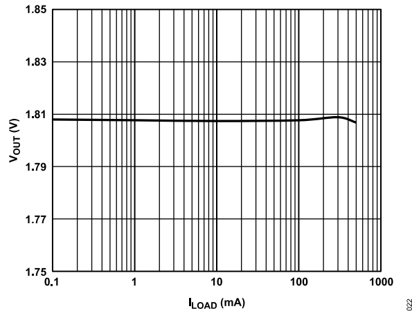
Figure 24. Output Voltage ( V_{OUT} ) vs. Load Current ( I_{LOAD} ), V_{OUT} = 1.8\text{ V}
