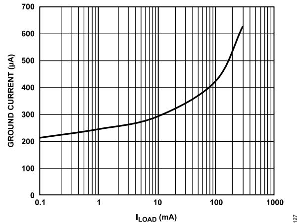
Figure 27. Ground Current ( I_{GND} ) vs. Load Current ( I_{LOAD} ), V_{OUT} = 1.8\text{ V}
