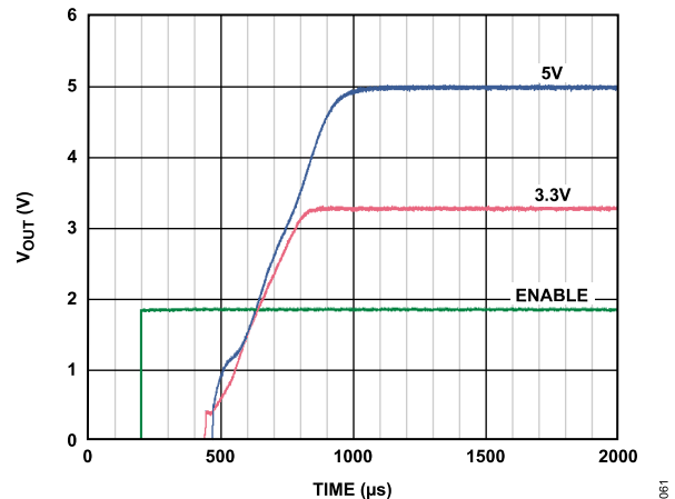
Figure 66. Typical Start-Up Behavior
