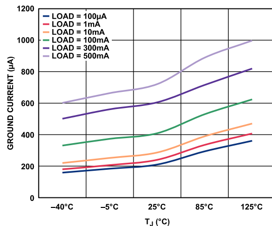
Figure 8. Ground Current ( I_{GND} ) vs. Junction Temperature ( T_J ), V_{OUT} = 3.3\text{ V}
