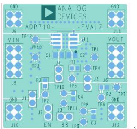
Figure 79. Example SOIC PCB Layout
