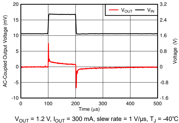
Figure 6-33. Line Transient
