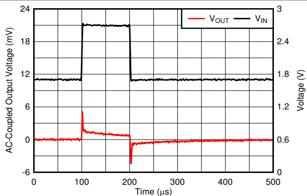
Figure 6-27. Line Transient
