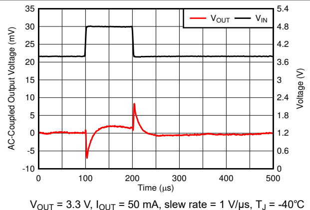
Figure 6-36. Line Transient
