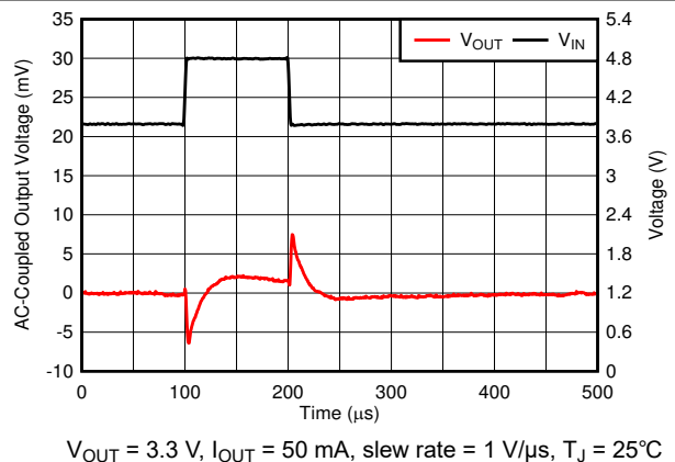
Figure 6-35. Line Transient
