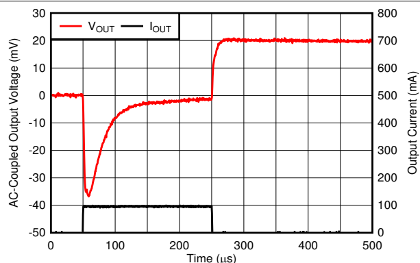
Figure 6-56. Load Transient
