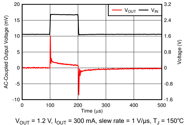
Figure 6-34. Line Transient
