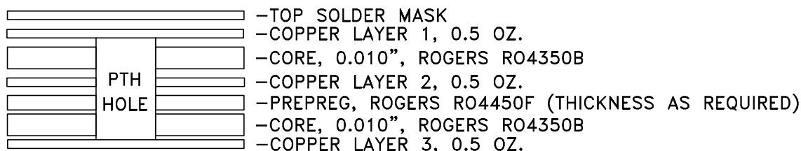
Stack-up Diagram
