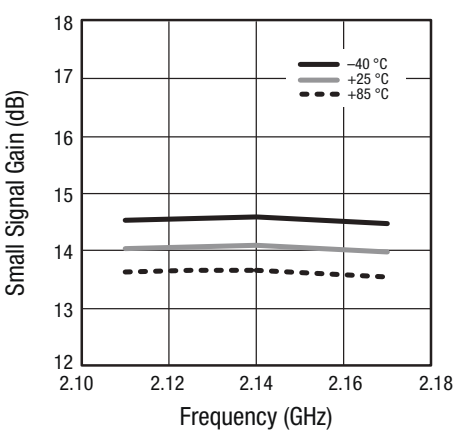
Figure 44. Small Signal Gain vs Frequency Over Temperature
