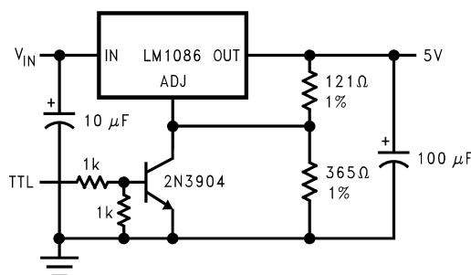
Figure 20. 5-V Regulator with Shutdown
