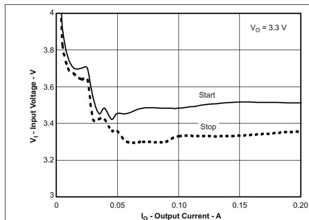
Figure 27. 3.3V Start/Stop Voltage
