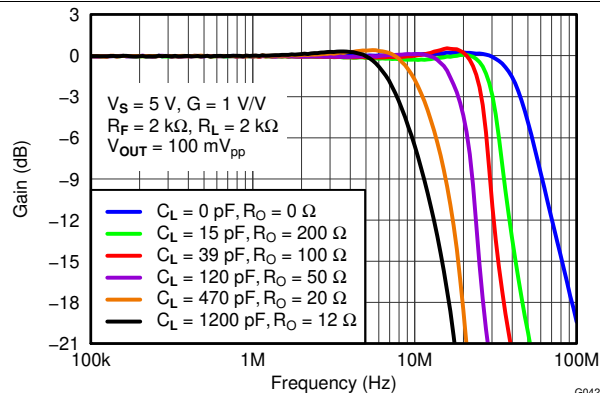
Figure 51. Frequency Response vs C_{LOAD}
