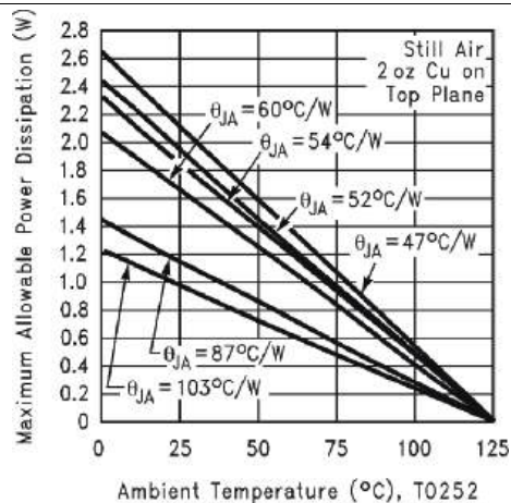
Figure 40. Maximum Allowable Power Dissipation vs Ambient Temperature for TO-252
