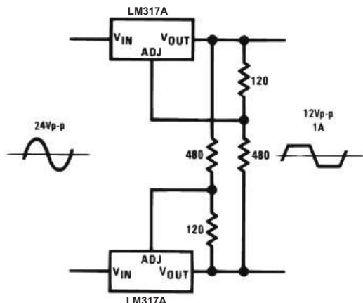
Figure 31. AC Voltage Regulator
