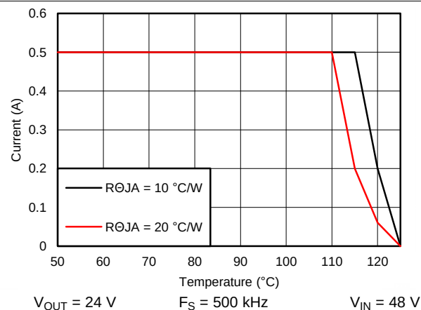
Figure 82. Derating Curve
