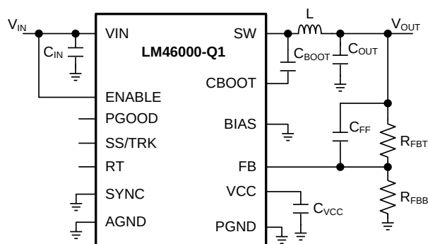
Figure 45. LM46000-Q1 Basic Schematic for V_{OUT} < 3.3 V, Tie BIAS to Ground
