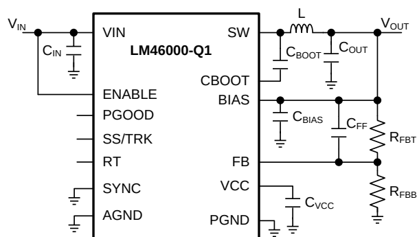
Figure 44. LM46000-Q1 Basic Schematic for V_{OUT} \geq 3.3 V, Tie BIAS to V_{OUT}
