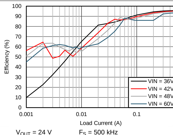
Figure 78. Efficiency
