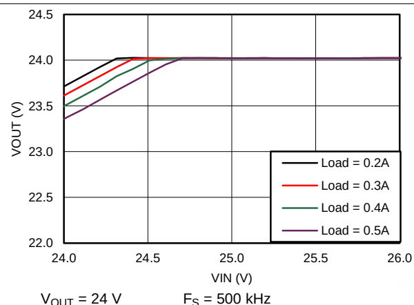
Figure 80. Dropout Curve
