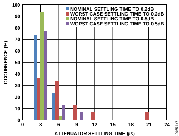
Figure 48. Attenuator Settling Time to 0.2 dB and 0.5 dB Distribution at Nominal and Worst-Case Conditions for Worst-Case Small Step (36 dB to 42 dB)
