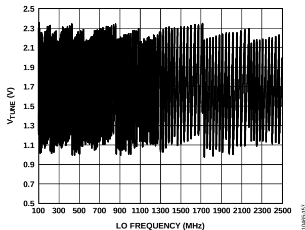
Figure 56. V_{TUNE} vs. LO Frequency
