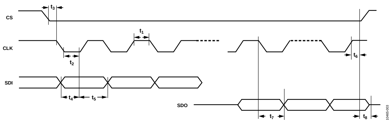
Figure 3. SPI Port Timing Diagram
