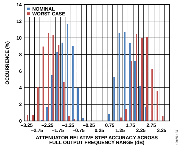
Figure 39. Attenuator Relative Step Accuracy Across Full Output Frequency Range Distribution at Nominal and Worst-Case Conditions, LO > 300 MHz, All Attenuation Steps
