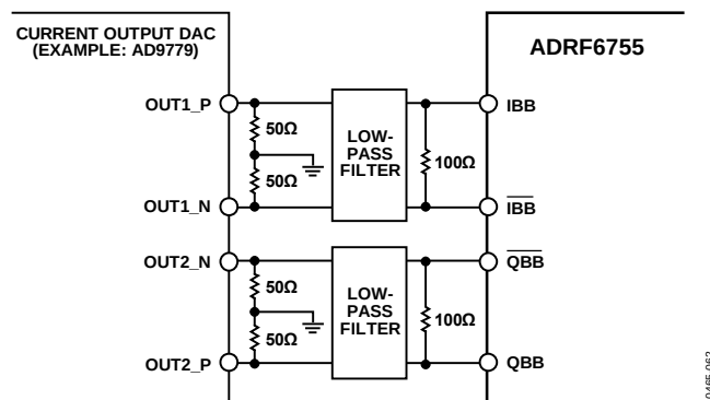
Figure 62. Typical Baseband Input Configuration
