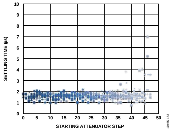
Figure 43. Attenuator Settling Time to 0.2 dB for Small Steps (1 dB to 6 dB) at Nominal Conditions
