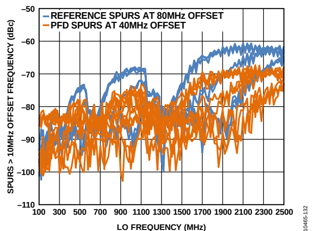
Figure 34. Spurs &gt; 10 MHz from Carrier vs. LO Frequency, Supply, and Temperature
