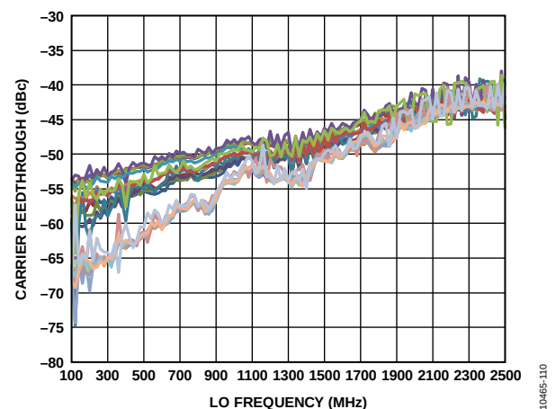
Figure 9. LO Carrier Feedthrough vs. LO Frequency, Attenuation, Supply, and Temperature
