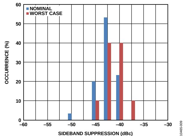
Figure 8. Sideband Suppression Distribution at Nominal and Worst-Case Conditions
