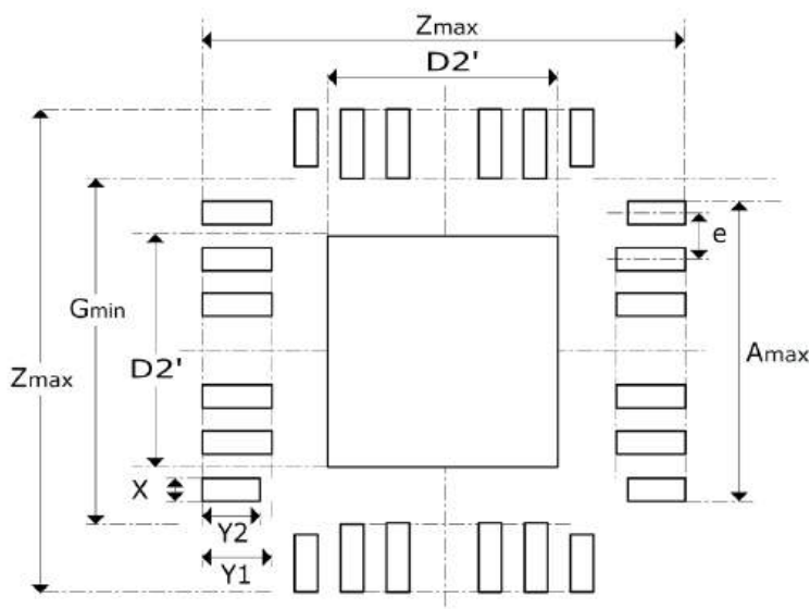
Figure 2.9 Pad Layout
