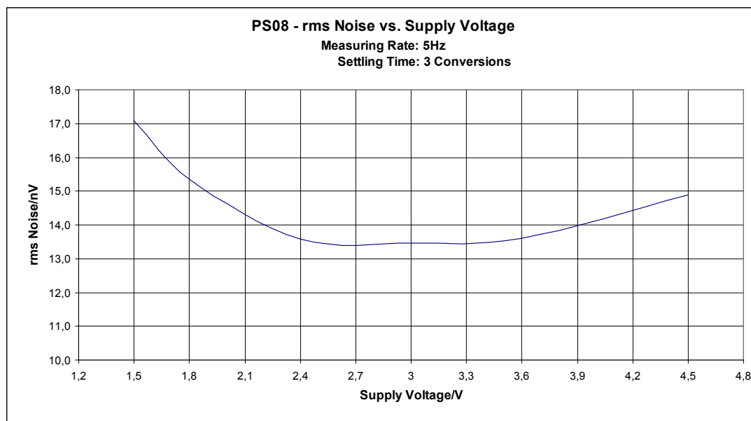
Figure 2.4 RMS-noise vs. supply voltage
