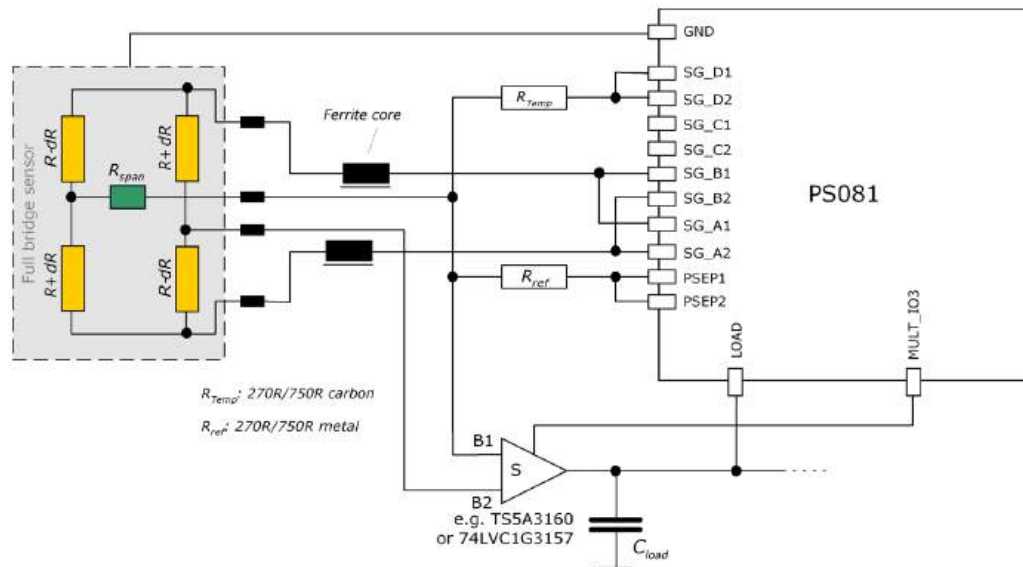
Figure 3.7 Connecting a Wheatston bridge
