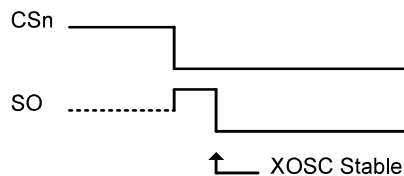
Figure 26: Power-On Reset
