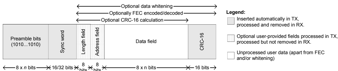
Figure 19: Packet Format
