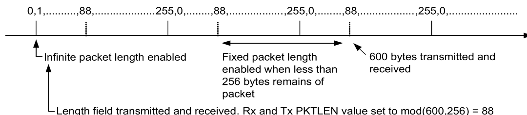
Figure 20: Packet Length > 255
