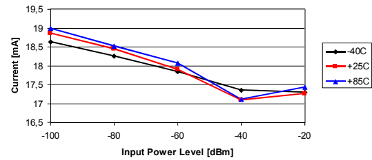
250 kBaud GFSK
