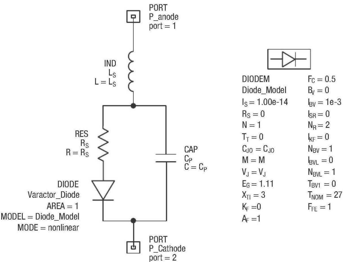
Figure 2. SPICE Model
