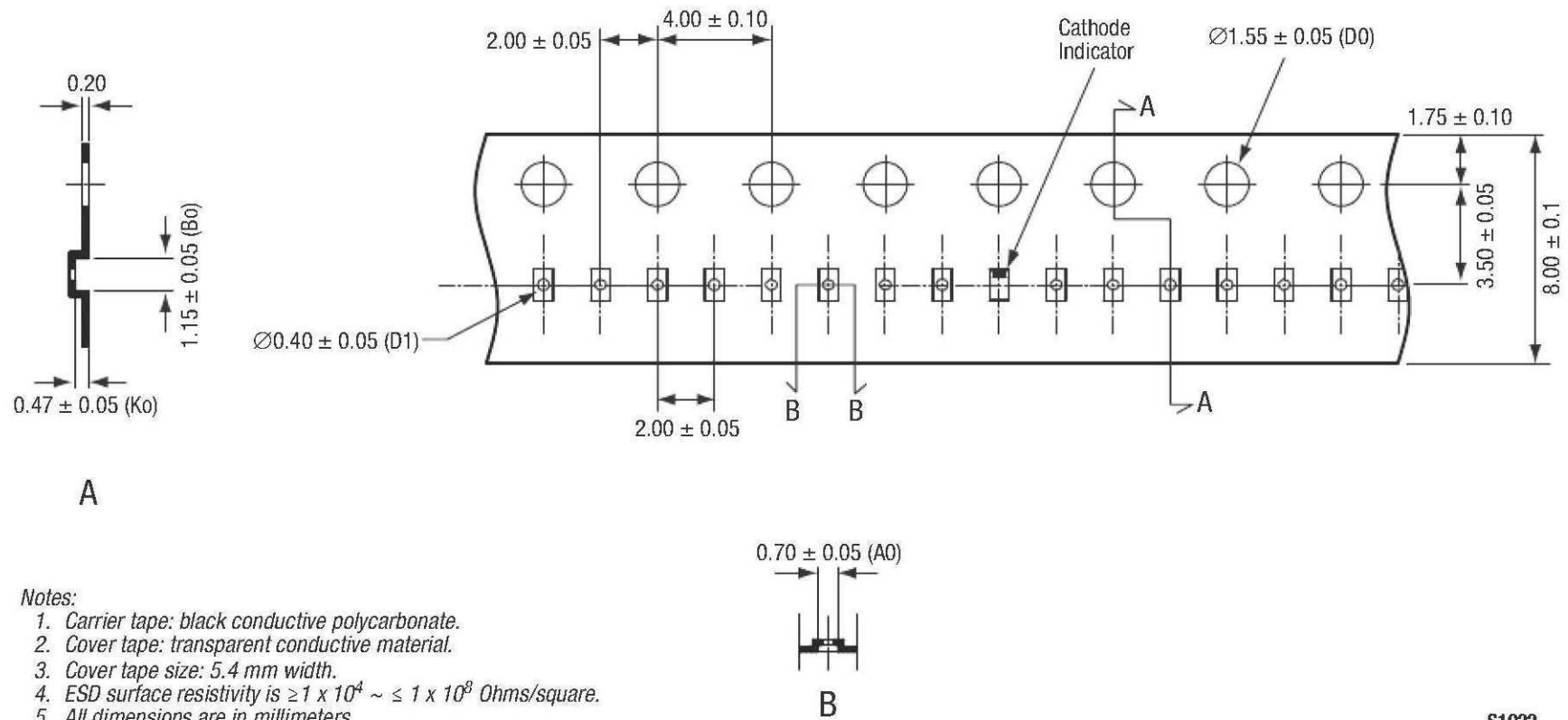
Figure 6. SOD-882 Tape and Reel Dimensions
