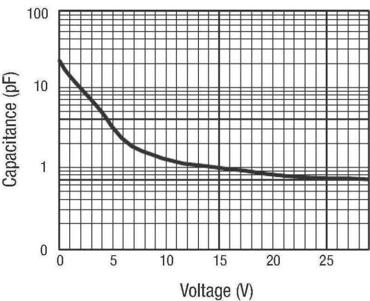
Figure 1. Capacitance vs Voltage @ 25 °C
